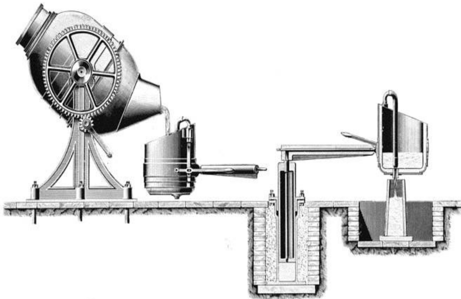
FIG. 44. EARLY FORM OF BESSEMER CONVERTING PLANT AT SHEFFIELD
